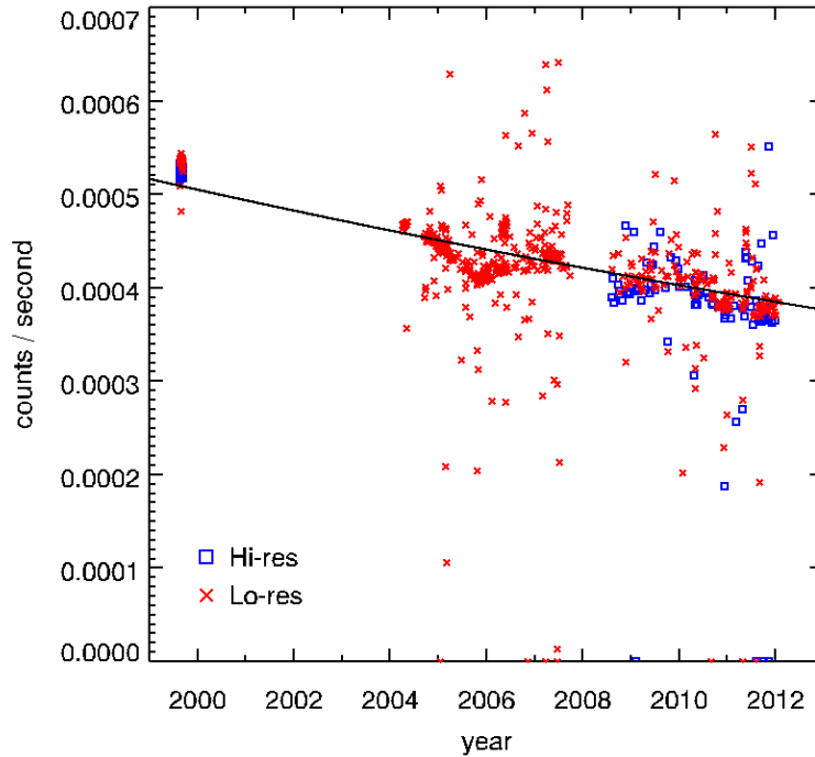
Figure 3.1 – Background count rate in the FUV detector as a function of time.
