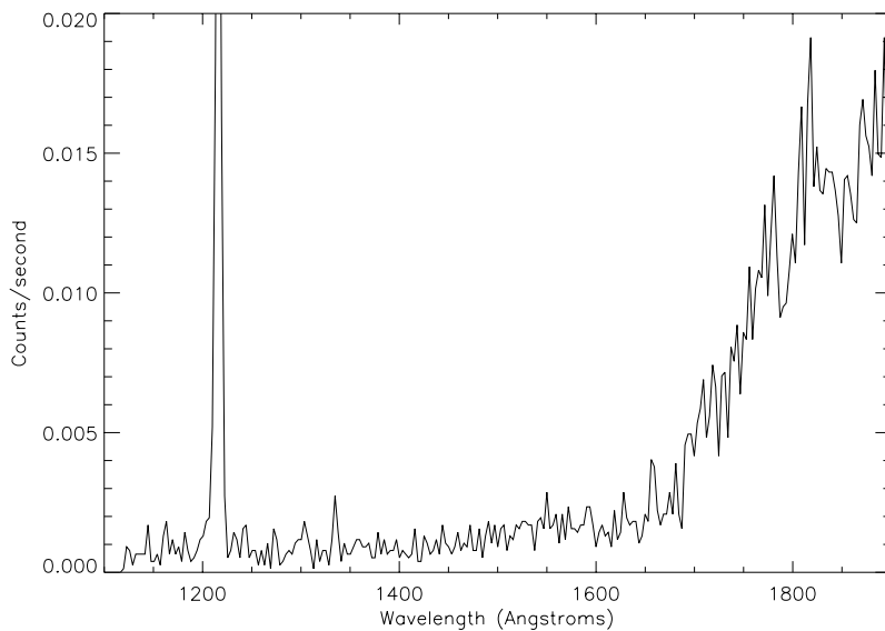
Figure 1.2: 2004 UVIS observation of Phoebe's dayside.
