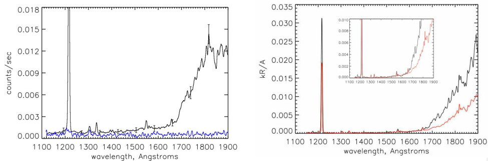
Figure 8.3. Sample spectra from Phoebe (phase angle \zeta = 42^\circ ). (left) Average raw spectrum (counts/s) from the dayside (average of 1224 spectra) and nightside background spectrum (in blue), with sample 1-\sigma statistical error bars shown. (right) Average calibrated spectrum ( kR/\text{\AA} ), nightside background subtracted, with scaled solar spectrum overplotted (in red). The solar spectrum has been scaled by fitting to the reflected 1335 \text{\AA} C II feature in the Phoebe spectrum.
