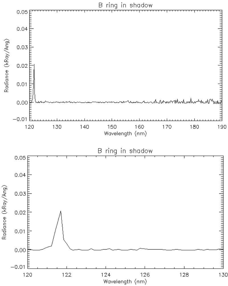
Figure 7.5 Radiance from an observation of the B ring while in Saturn's shadow. The upper panel shows the full spectral extent of the FUV channel while the lower panel shows only the spectra from 120-130 nm. Lyman- \alpha scattering at longer wavelength pixels is negligible except for wavelengths less than 1 nm from line center. If the goal of an investigator is to measure Lyman- \alpha reflectance from the rings, then the radiance over the entire broadened spectral line must be summed and multiplied by the bandpass of the instrument.
