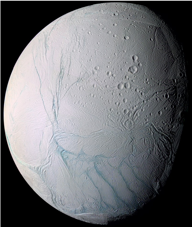
ISS mosaic
