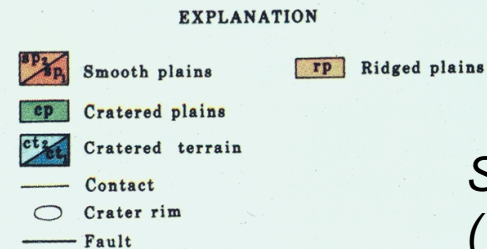
ENCELADUS GEOLOGIC-TERRAIN MAP
