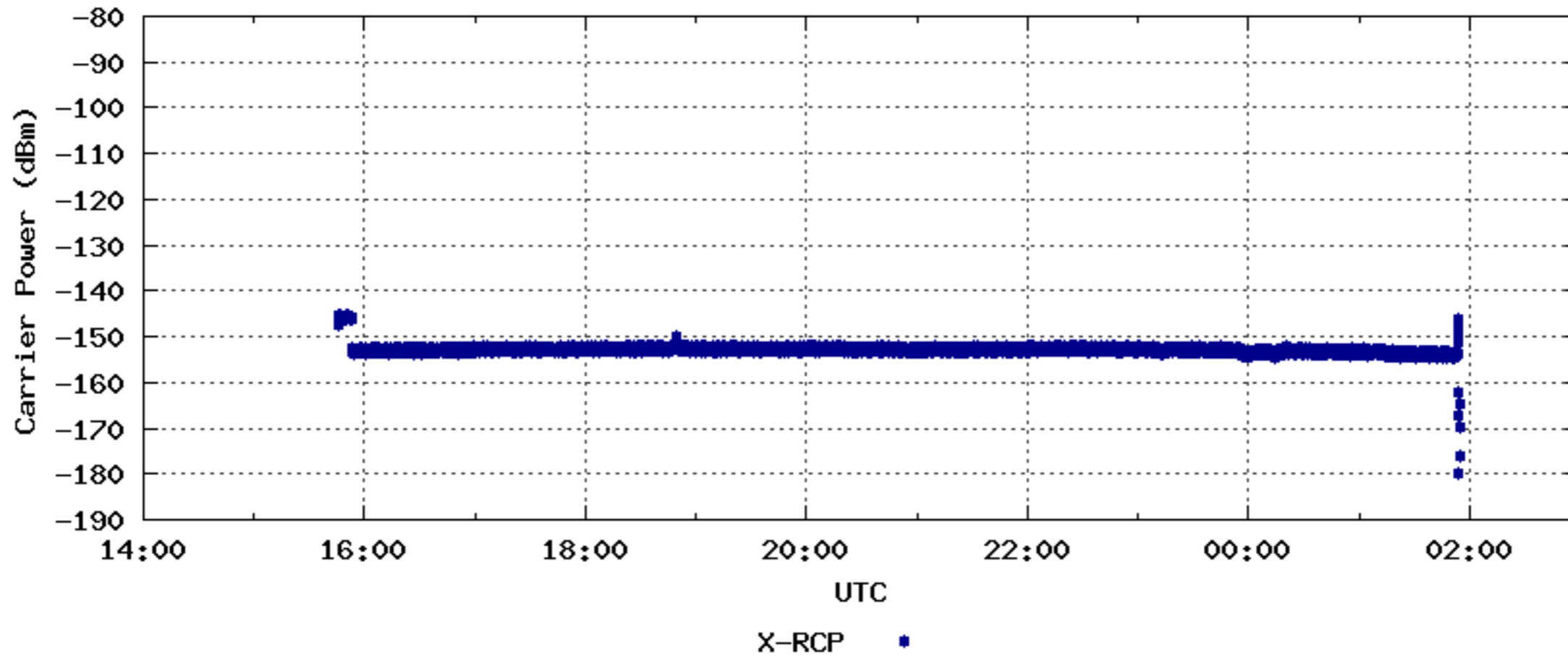
2005/178 DSS-15 Carrier Power
