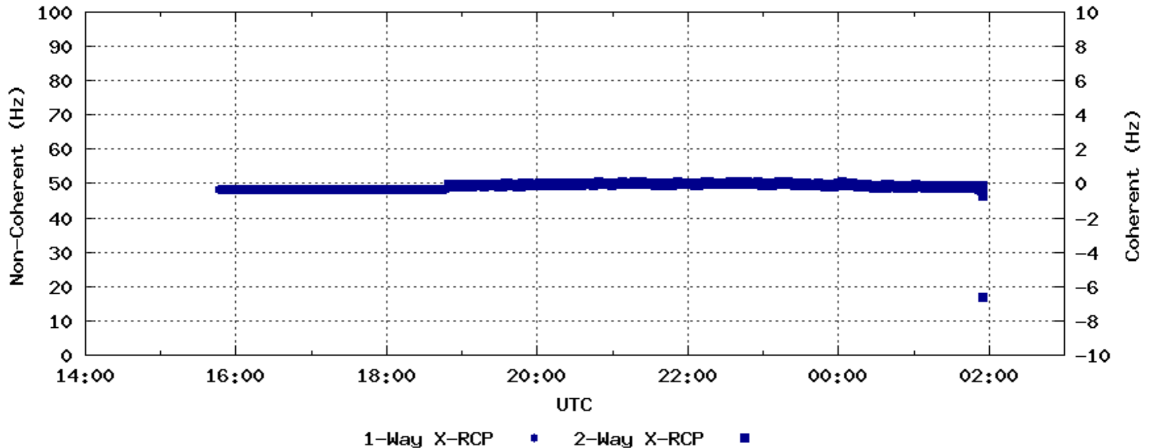
2005/178 DSS-15 X-Band Residual Frequency (Measured - Predicted)
