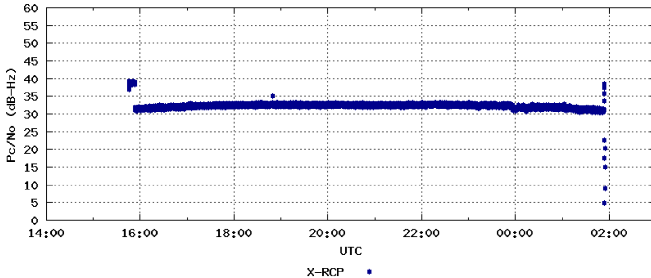
2005/178 DSS-15 Carrier Power to Noise Spectral Density Ratio (Pc/No)
