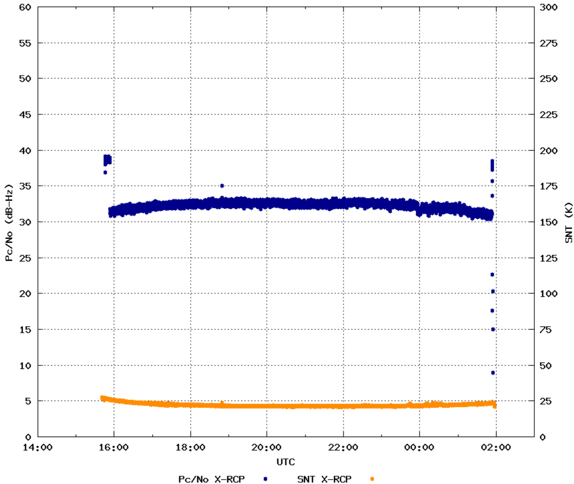
2005/178 D55-15 Carrier Power to Noise Spectral Density Ratio and System Noise Temperature
