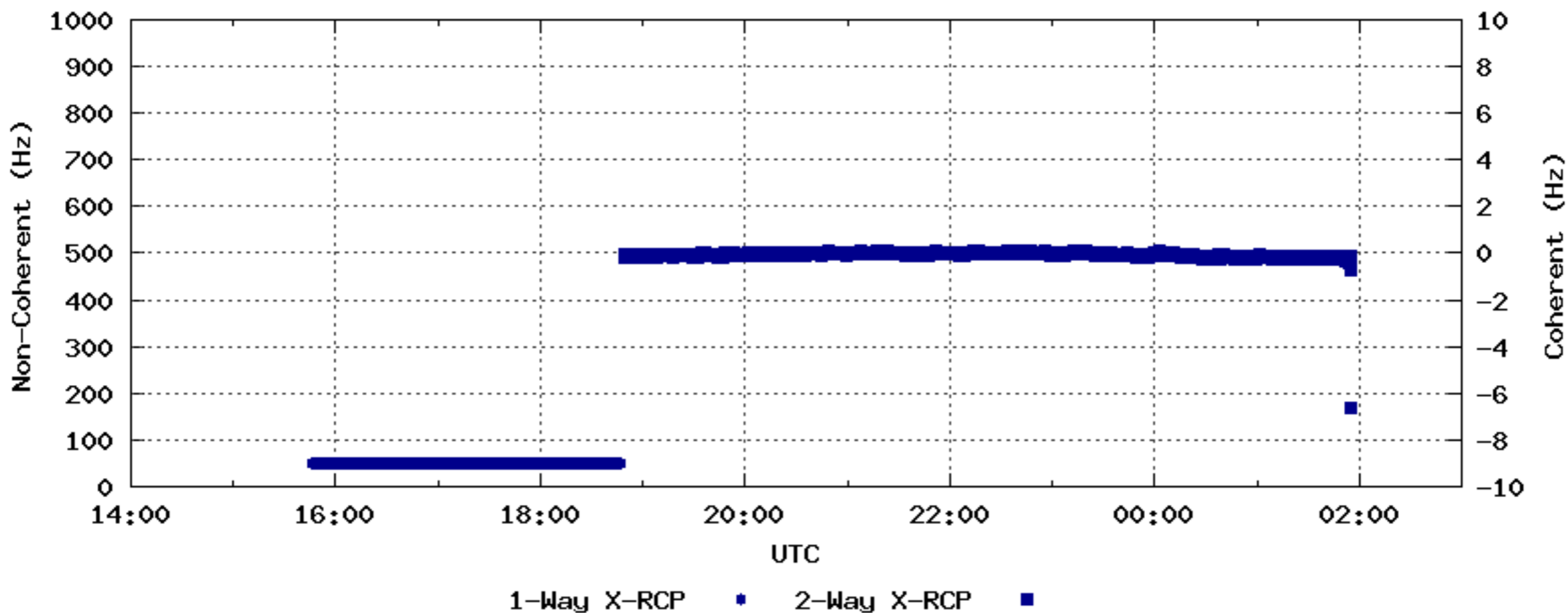
2005/178 D55-15 Carrier Frequency Residual (Measured - Predicted)
