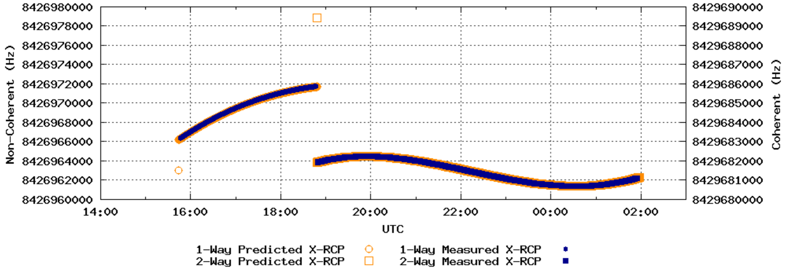
2005/178 DSS-15 X-Band Measured and Predicted Carrier Frequency
