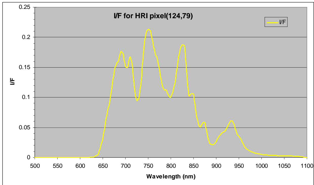
Figure 5.8-17: Expanded view of I/F for HRI pixel(124,79) from 134 km altitude.
