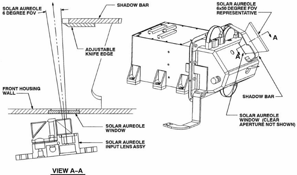
Figure 5.9-2: Layout and Field of View of the DISR SA cameras.
